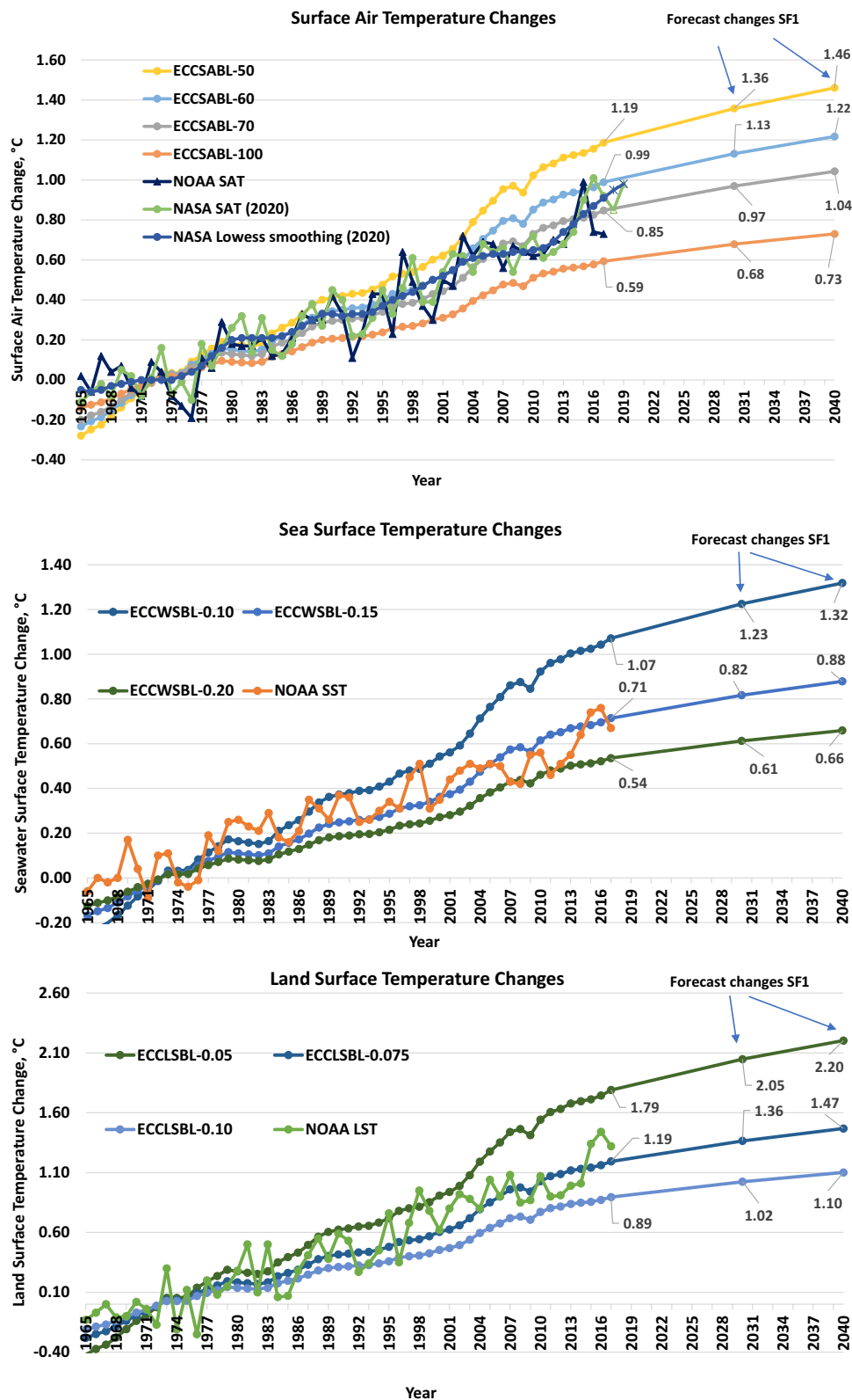
Fig. 3 Calculated past temperature changes at the lower and upper depth limits of equivalent climate change surface air boundary layer (top), equivalent climate change waters surface boundary layer (middle), and equivalent climate change land surface boundary layer (bottom), and the temperature change forecast as well as their observed temperature anomalies under scenario SF1
