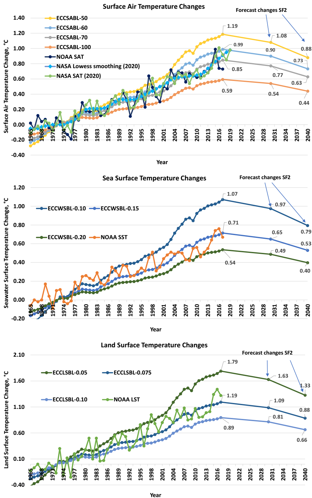
Fig. 4 Calculated past temperature changes at the lower and upper depth limits of equivalent climate change surface air boundary layer (top), equivalent climate change waters surface boundary layer (middle), and equivalent climate change land surface boundary layer (bottom), and the temperature change forecast as well as their observed temperature anomalies under scenario SF2
